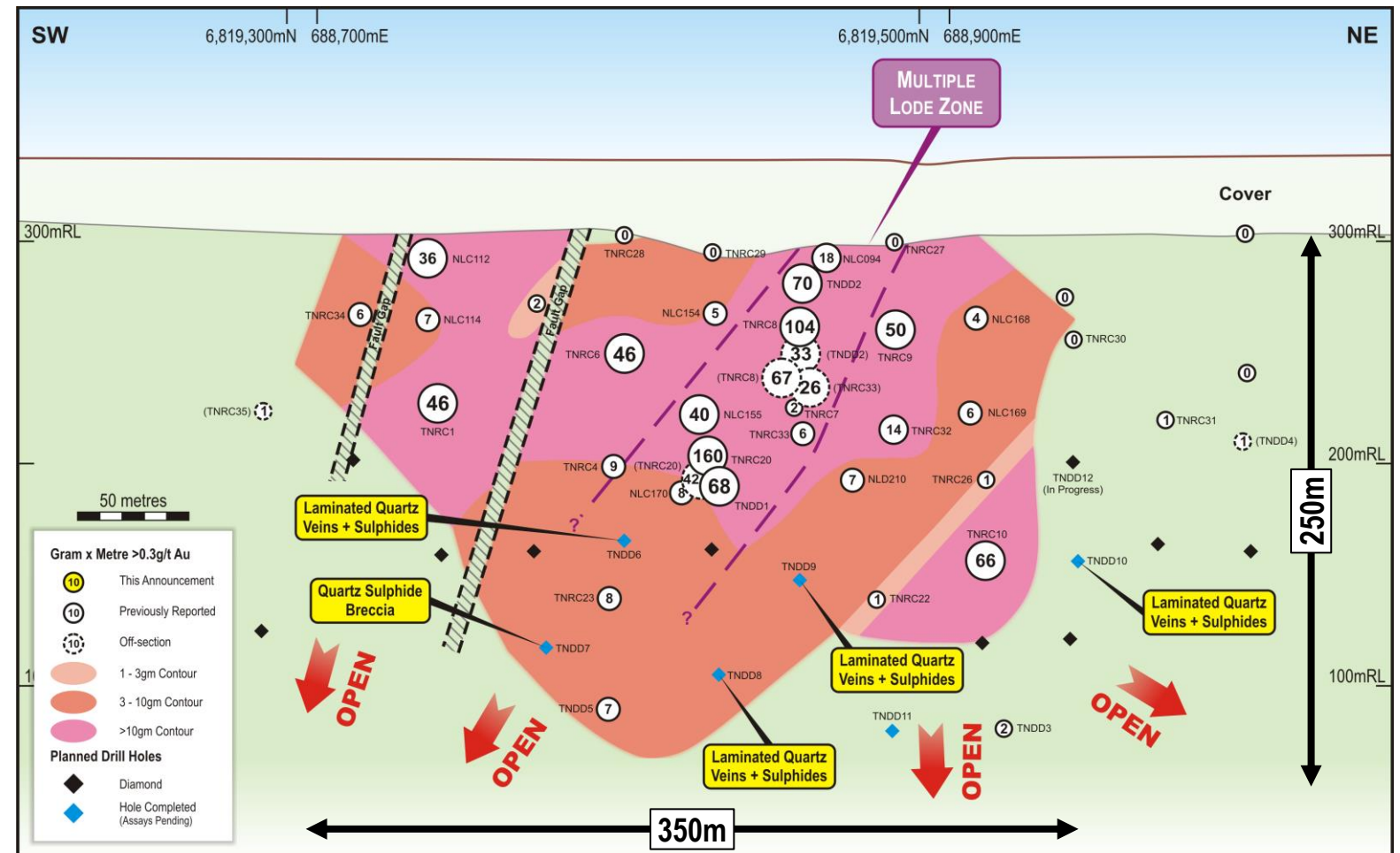
Hercules prospect long section showing significant gram-metre gold intervals and contours (interval grade (g/t Au) x width (m))
